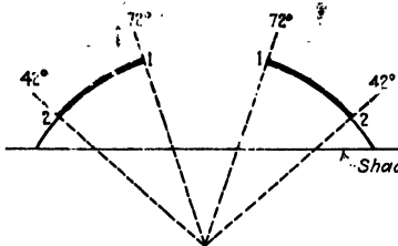
FIG. 12.—Basal plane (00·1) diffraction arcs. X-ray beam 8° to rolling plane, 90° to rolling direction.
